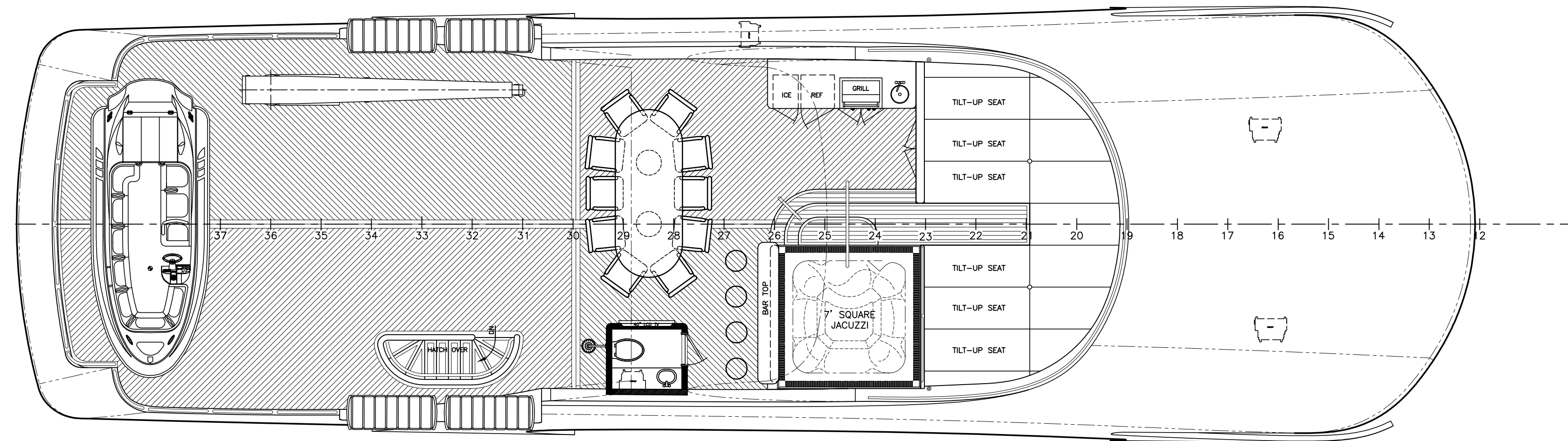
02 DECK OPTION 1
