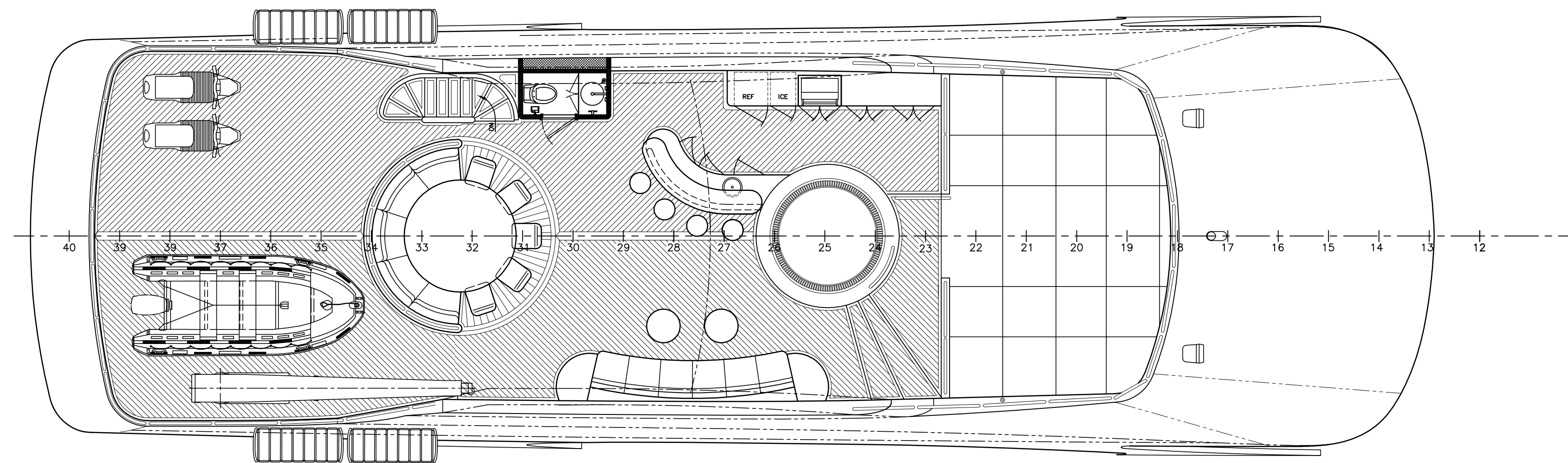
02 DECK OPTION 3
