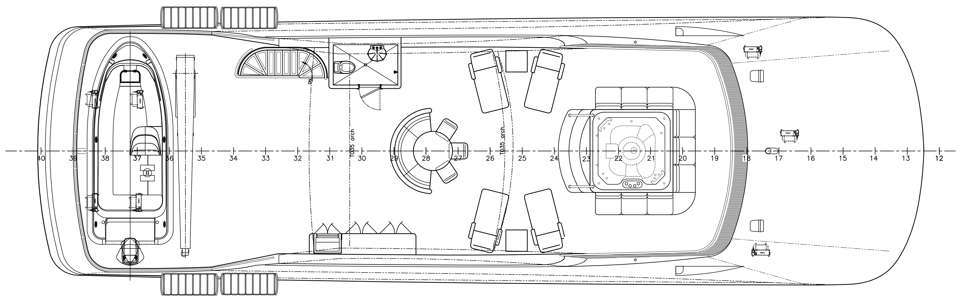
FLYBRIDGE OPTION #2
