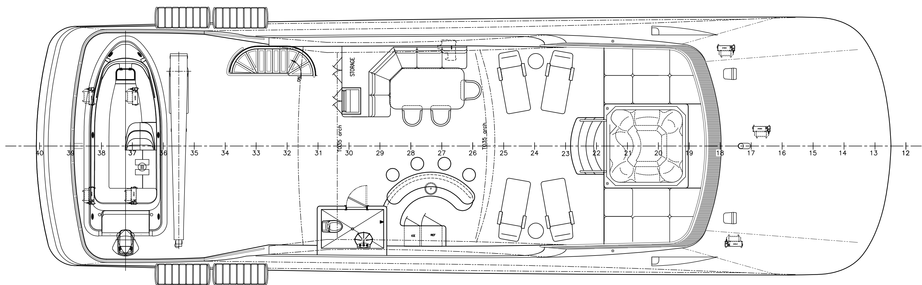
FLYBRIDGE OPTION #1
