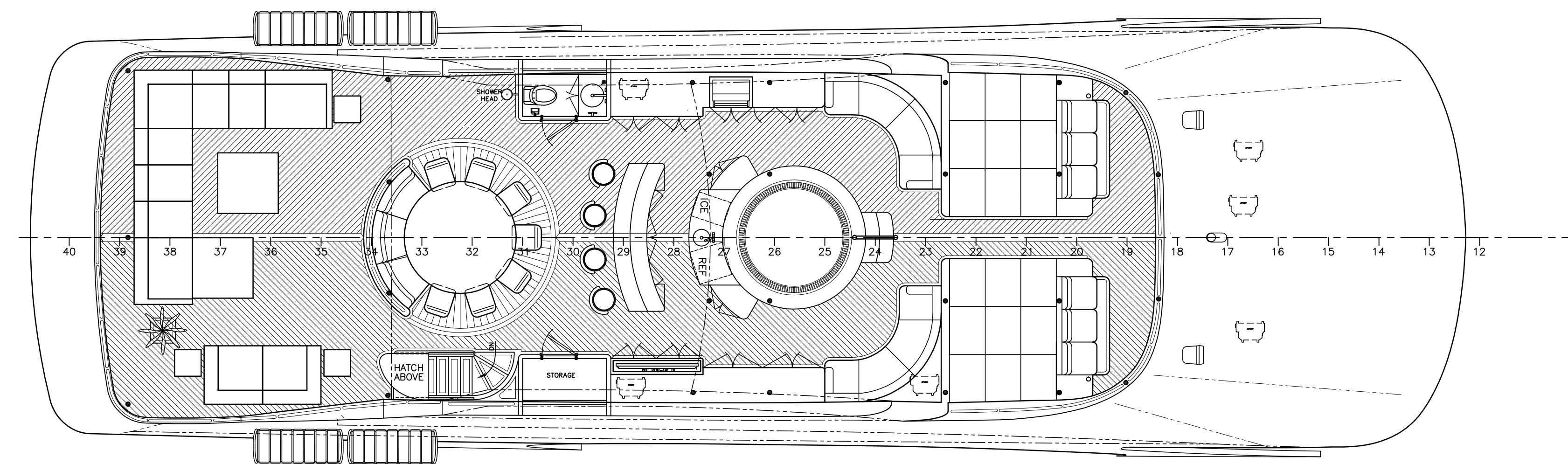
02 DECK OPTION 2
