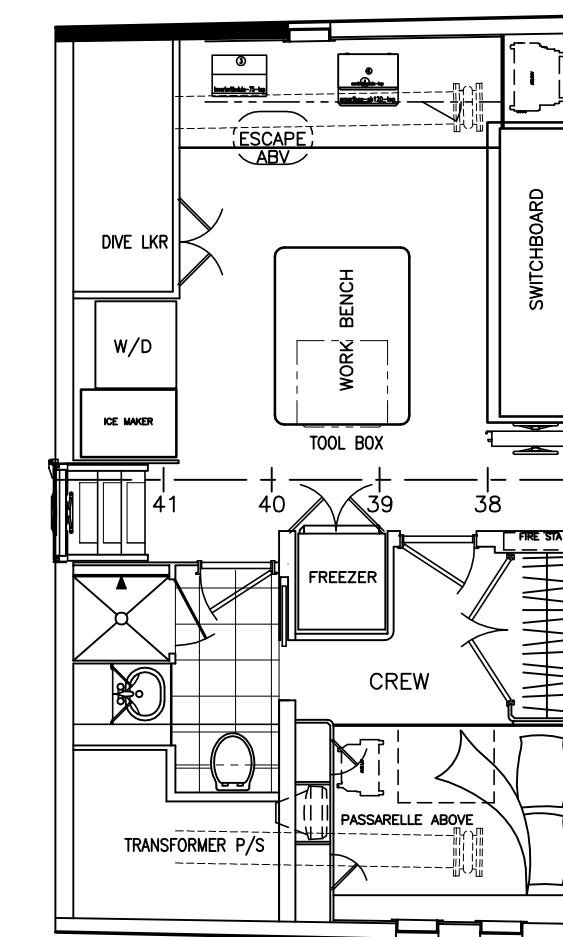
LAZARETTE OPTION
